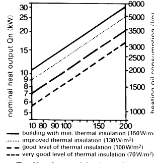
③ Heating and fuel requirements of houses in relation to insulation levels
